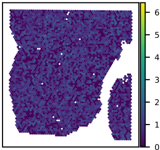
SNU25B FAM204A expression Moran's I = 0.01
