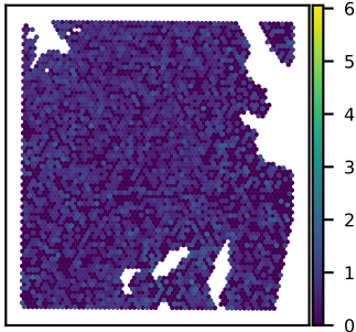
SNU51A SRP54 expression Moran's I = 0.02
