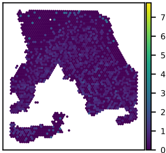
SNU18A C16orf70 expression Moran's I = 0.04
