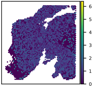
SNU24A DHCR7 expression Moran's I = 0.10
