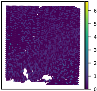
SNU43A HECTD2 expression Moran's I = 0.02
