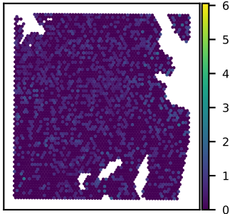
SNU51A CDC37L1 expression Moran's I = 0.01
