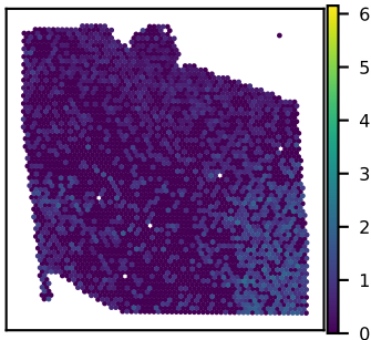
SNU27A C1orf216 expression Moran's I = 0.20
