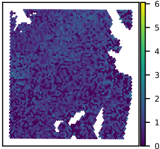
SNU51A CNPY3 expression Moran's I = 0.09
