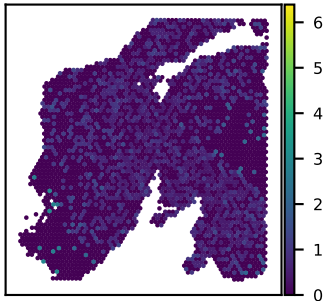
SNU24A TMEM161A expression Moran's I = 0.03
