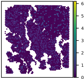
SNU16B CENPN expression Moran's I = 0.02
