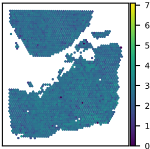
SNU25A HNRNPDL expression Moran's I = 0.09
