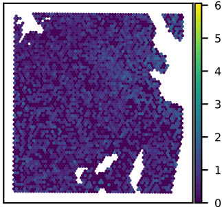
SNU51A GDAP1 expression Moran's I = 0.06
