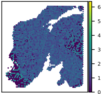
SNU24A PYURF expression Moran's I = 0.08
