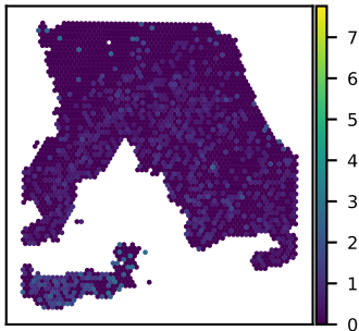
SNU18A CDKN2D expression Moran's I = 0.11
