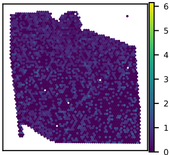
SNU27A SPECC1L expression Moran's I = 0.01
