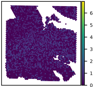
SNU24B KLHL25 expression Moran's I = 0.05
