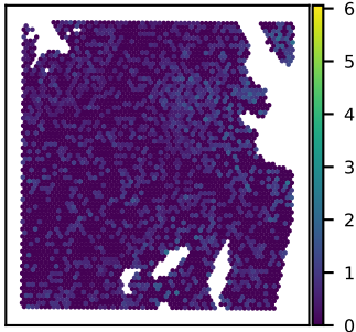
SNU51A SEZ6L2 expression Moran's I = 0.08
