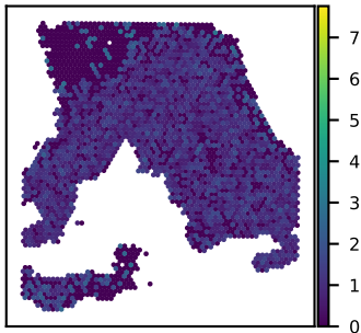
SNU18A ENTPD6 expression Moran's I = 0.11
