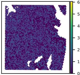
SNU51A KCTD5 expression Moran's I = 0.02
