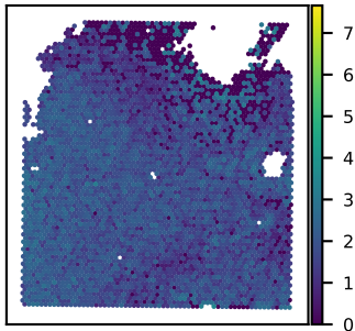
SNU21B ZCCHC24 expression Moran's I = 0.33
