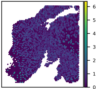
SNU24A NCOA3 expression Moran's I = 0.05
