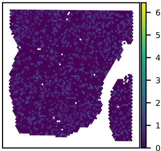
SNU25B SLC35B4 expression Moran's I = 0.01
