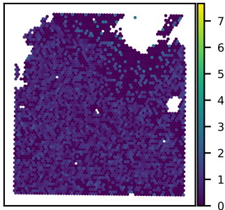
SNU21B TMEM101 expression Moran's I = 0.03
