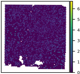
SNU43A SLC25A26 expression Moran's I = -0.01
