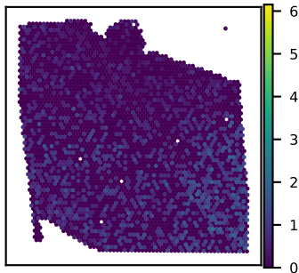
SNU27A RASGRF2 expression Moran's I = 0.08
