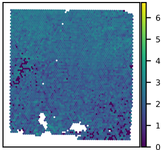
SNU43A SERPINA3 expression Moran's I = 0.28
