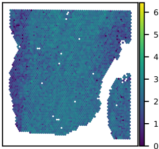
SNU25B TMEM59L expression Moran's I = 0.46
