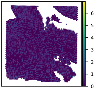
SNU24B SMYD3 expression Moran's I = 0.03
