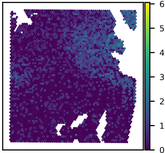
SNU51A INPP5F expression Moran's I = 0.42
