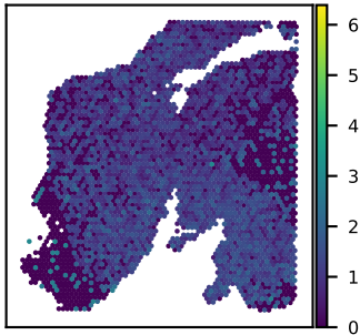
SNU24A C2orf80 expression Moran's I = 0.18
