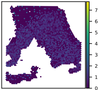
SNU18A TMEM176A expression Moran's I = 0.14
