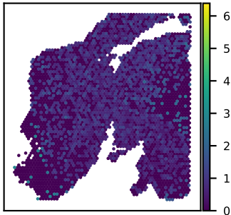
SNU24A CLEC2D expression Moran's I = 0.06
