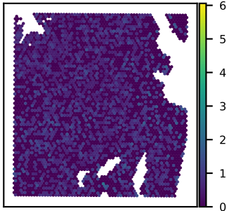
SNU51A PPWD1 expression Moran's I = 0.01
