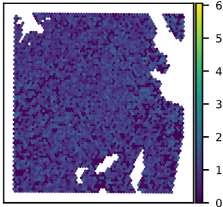
SNU51A SLC30A9 expression Moran's I = 0.03
