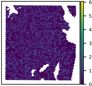
SNU51A TMEM185B expression Moran's I = 0.02
