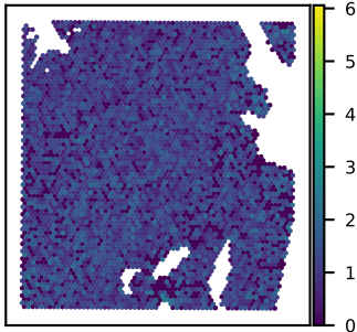
SNU51A BABAM1 expression Moran's I = 0.04
