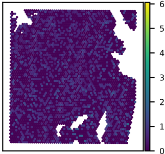
SNU51A NDUFAB5 expression Moran's I = 0.01
