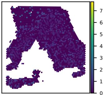
SNU18A KCTD15 expression Moran's I = 0.03
