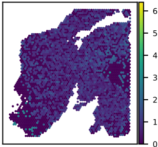
SNU24A EFHC1 expression Moran's I = 0.09
