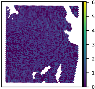
SNU51A ITGB1BP1 expression Moran's I = 0.01
