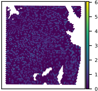
SNU51A TSPAN12 expression Moran's I = 0.02
