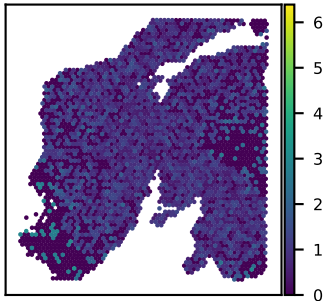
SNU24A GLOD4 expression Moran's I = 0.05
