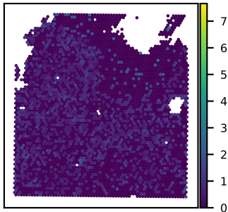
SNU21B INPP5A expression Moran's I = 0.07
