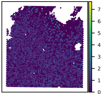
SNU21B ANKRD12 expression Moran's I = 0.04
