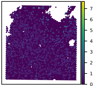
SNU21B TMEM216 expression Moran's I = 0.03
