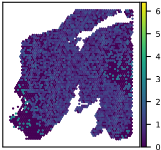
SNU24A ARFGAP3 expression Moran's I = 0.06
