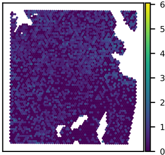
SNU51A FGF12 expression Moran's I = 0.09
