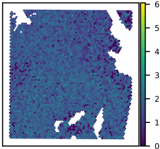
SNU51A EMC10 expression Moran's I = 0.14
