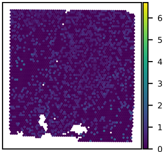
SNU43A CTDP1 expression Moran's I = 0.01
