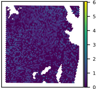
SNU51A TBC1D4 expression Moran's I = 0.05
